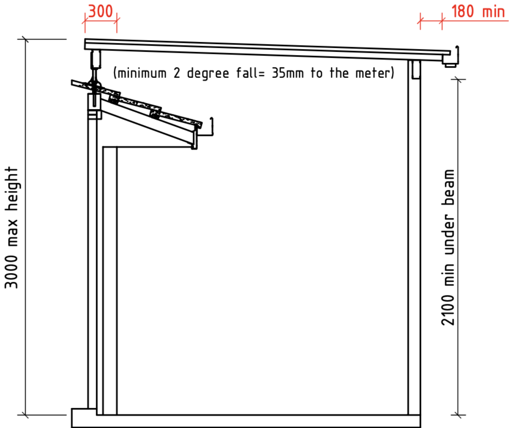
SIDE ELEVATION
